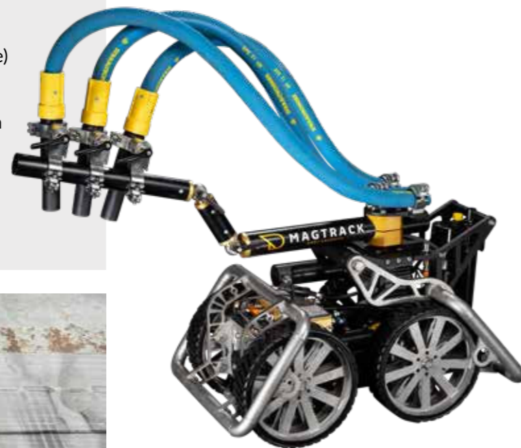
SANDBLASTER TILT SWING ARM
